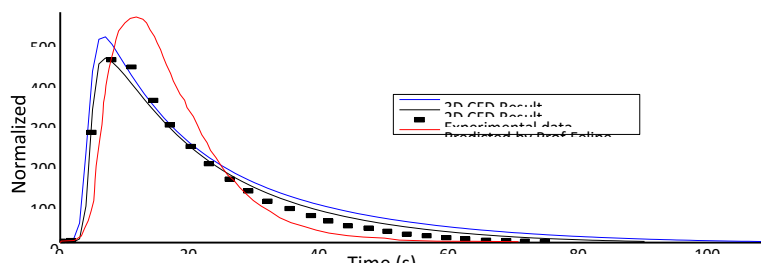
Figure 5. Experimental and predicted RTD response of the fluidized bed under normalized velocity conditions ( U_0/U_{mf} = 9.5 ).
