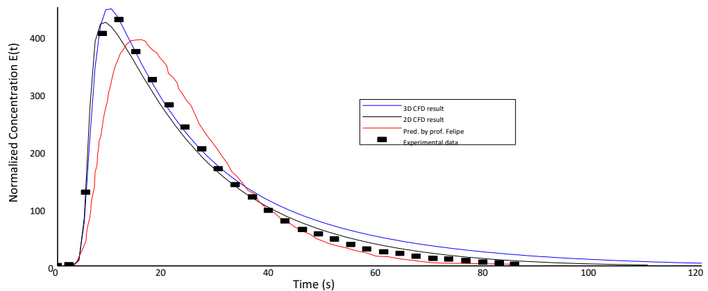
Figure 6. Experimental and predicted RTD response of the fluidized bed under normalized velocity conditions ( U_0 / U_{mf} \approx 8.0 ). 3D simulation results are in line with the experimental data (Figures 5 to 7, respectively) especially at lower simulation times; while it seems to over-predict the experimental data as the simulation time proceeds in the end. This is probably because of the numerical discrepancies associated with the CFD model while obtaining the final tracer concentration at the outlet. However, the peaks from the experimental data fit well with the numerical model, although the peaks from the 2D simulations are slightly lower than the peaks from the 3D simulations. This is probably because in 3D, tracer has enough space to pass through the fluidized bed.
