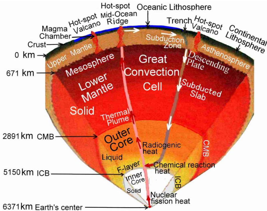
Figure 2. A schematic diagram of a great convection cell and heat flow, and the composition of Earth's interior.
