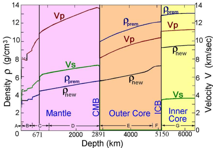
Figure 1. Seismic velocity and density in the Earth's interior of PREM and the new earth model.
