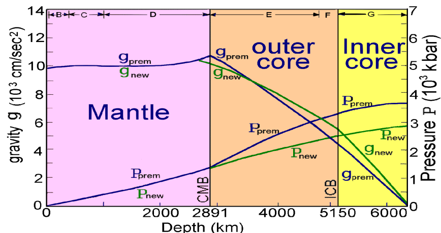
Figure 4. The Diagram of the gravity g and the pressure P compares between the new Earth model and the PREM. The average radius of Mars is 3397 km, the mass 642.40 \times 10^{24} g, and the average density 3.912 \text{ g/cm}^3 . Both values of the radius and the average density of the dark planet in the new Earth model are bigger than those of Mars, therefore, this model is found to be the more suitable one.
