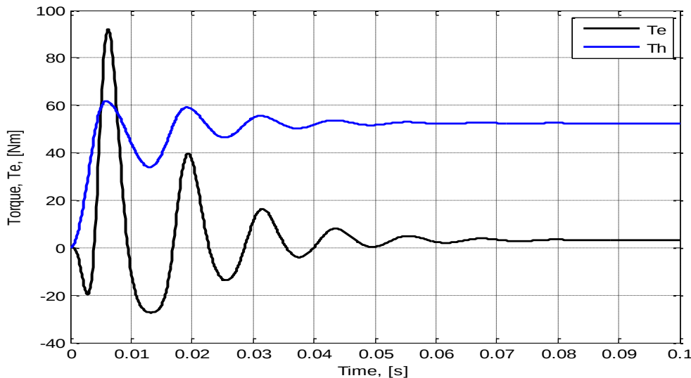
Figure 9: Graph of Torque against Time
