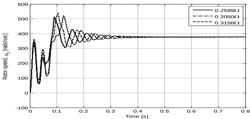
Figure 6: Graph of Rotor Speed against Time for Varying Stator Resistance.
