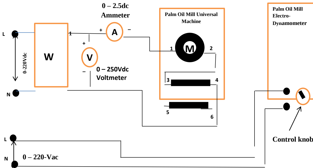
Figure4: Circuit diagram of industrial palm oil milling universal machine for uncompensated for DC operation.
