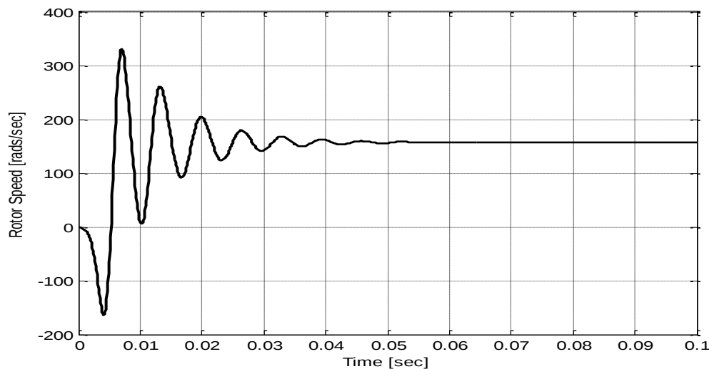
Figure 8: Graph of Rotor Speed against Time.
