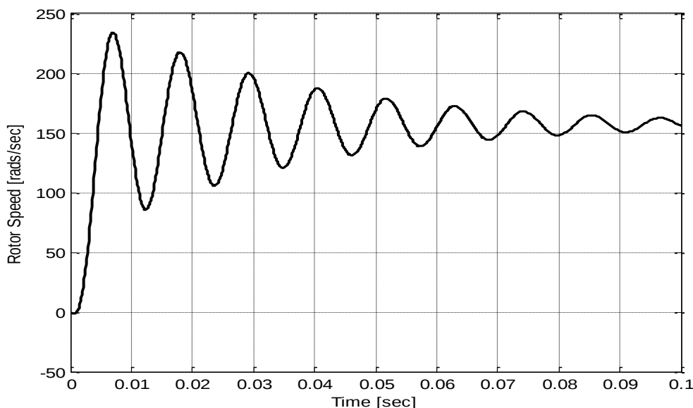
Figure 10: Graph of Rotor speed Against Time
