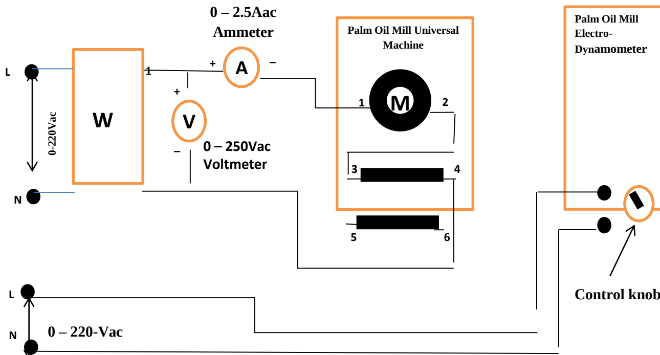
Figure3: Circuit diagram of industrial palm oil milling universal machine for uncompensated for AC operation.
