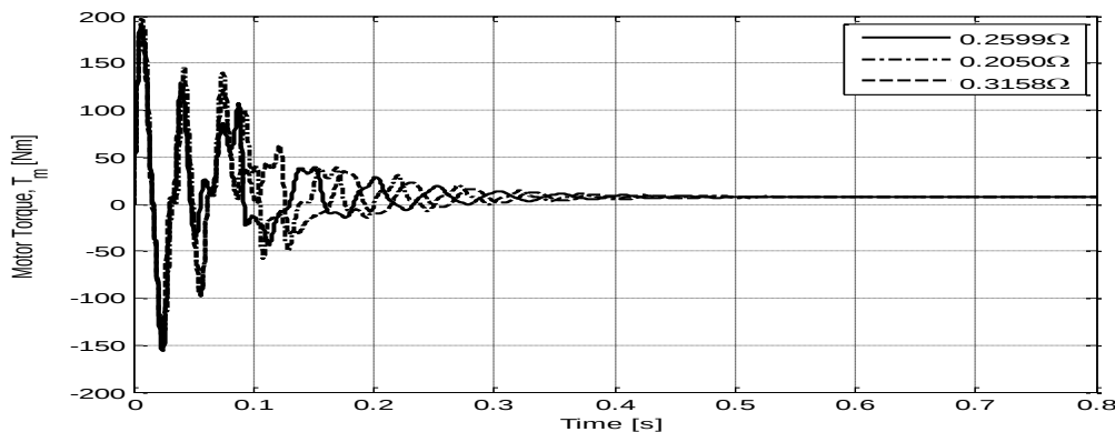
Figure 7.: Graph of Motor Torque against Time for Varying Stator Resistance
